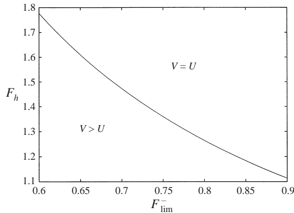
FIGURE 2. Froude number ranges for which the bore speed V is greater than or equal to the ship speed U .
